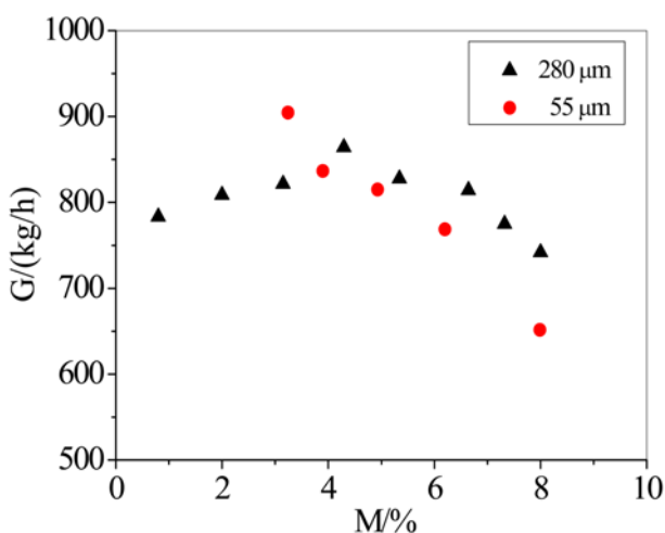
Fig. 6. Influence of moisture content on mass flow rate.
